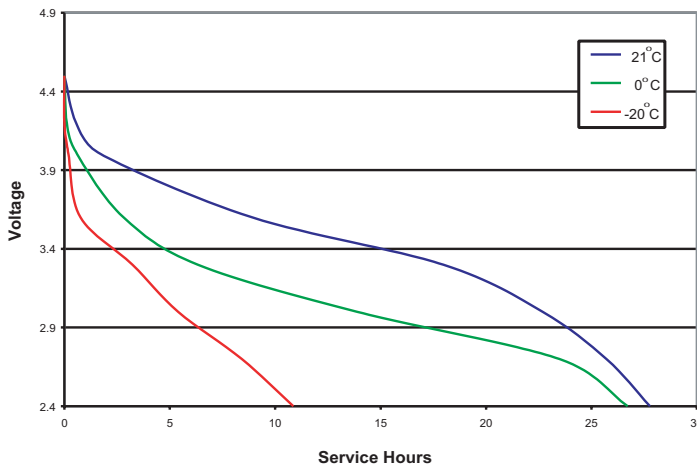
Typical Discharge at 20 ohm at various Temperatures
