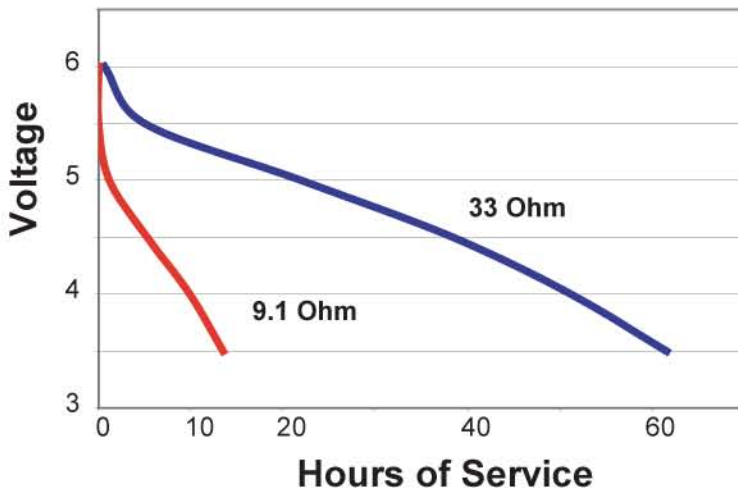
TYPICAL DISCHARGE CHARACTERISTICS AT 21°C
