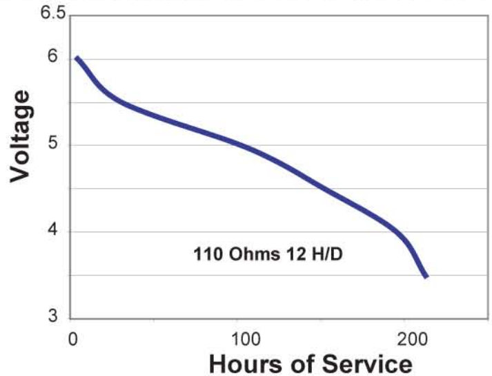
TYPICAL DISCHARGE CHARACTERISTICS AT 21°C
